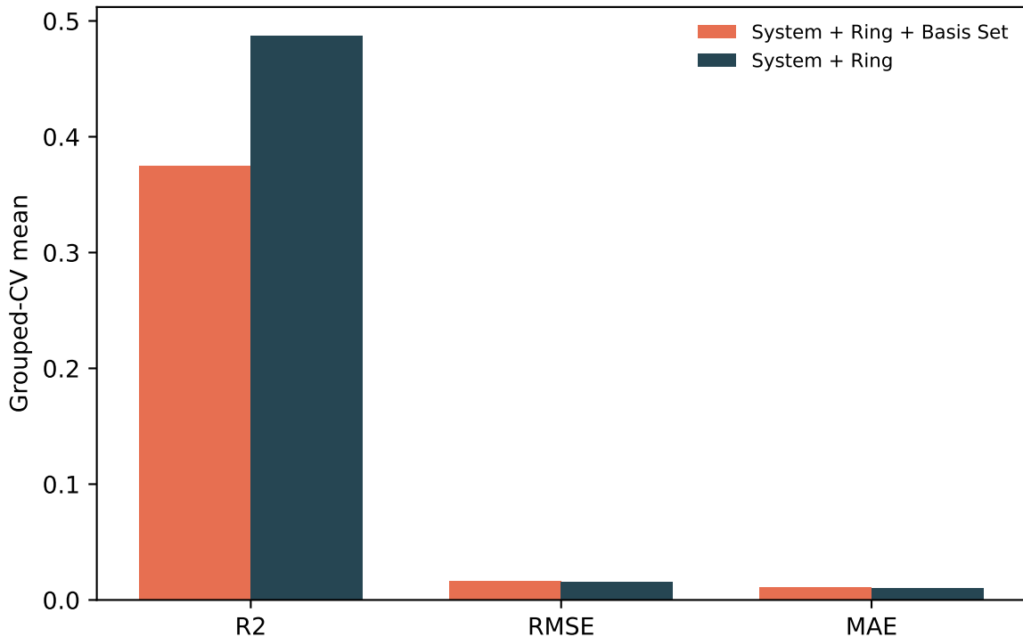
Ablation: norm, |Q_2|(0)
